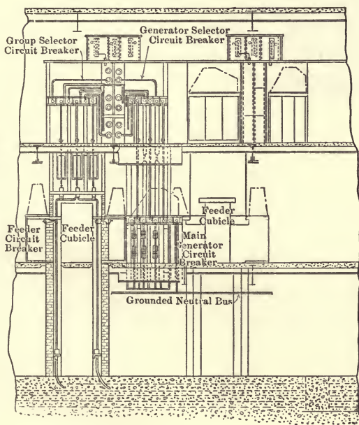
the power plant of the Long Island R. R. Co.
